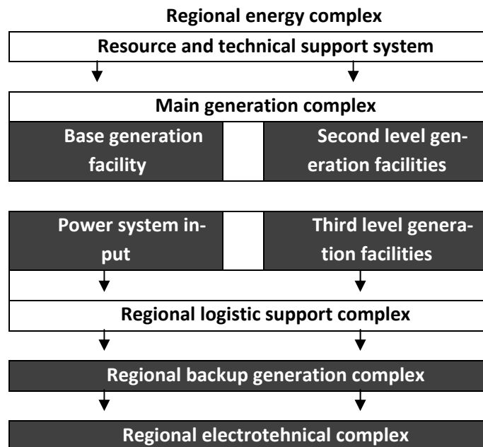
Fig. 1. The basic configuration and structure of regional power complex
