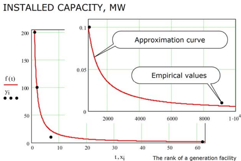
Fig. 2. The optimised parameter-based rank distribution of generation facilities in the power system of the Kaliningrad region (modelling results)
